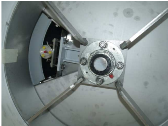
Old flanged bearing arrangement
